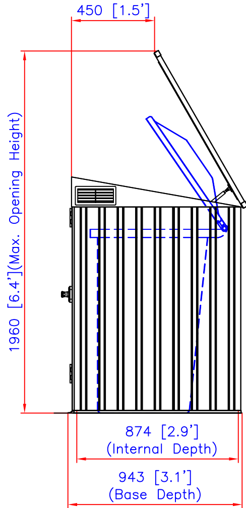
Side View (Door Opened)
