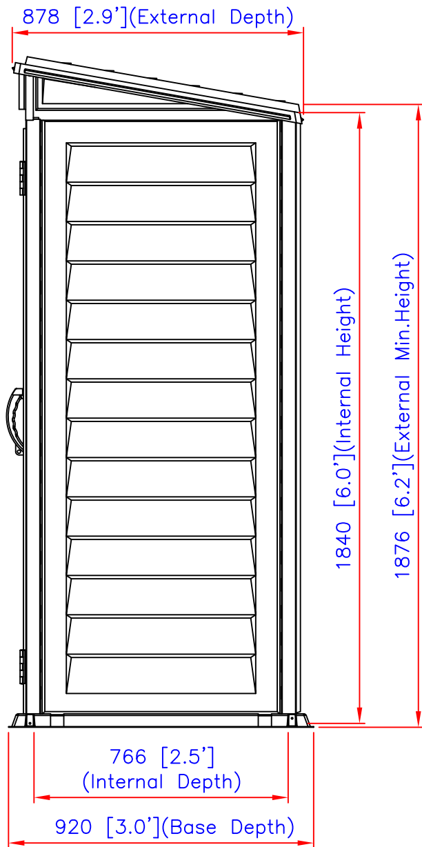
Side View
