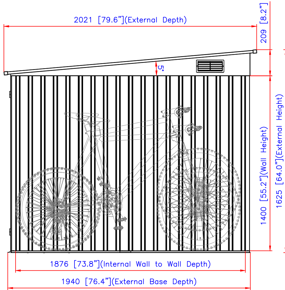
SIDE VIEW
