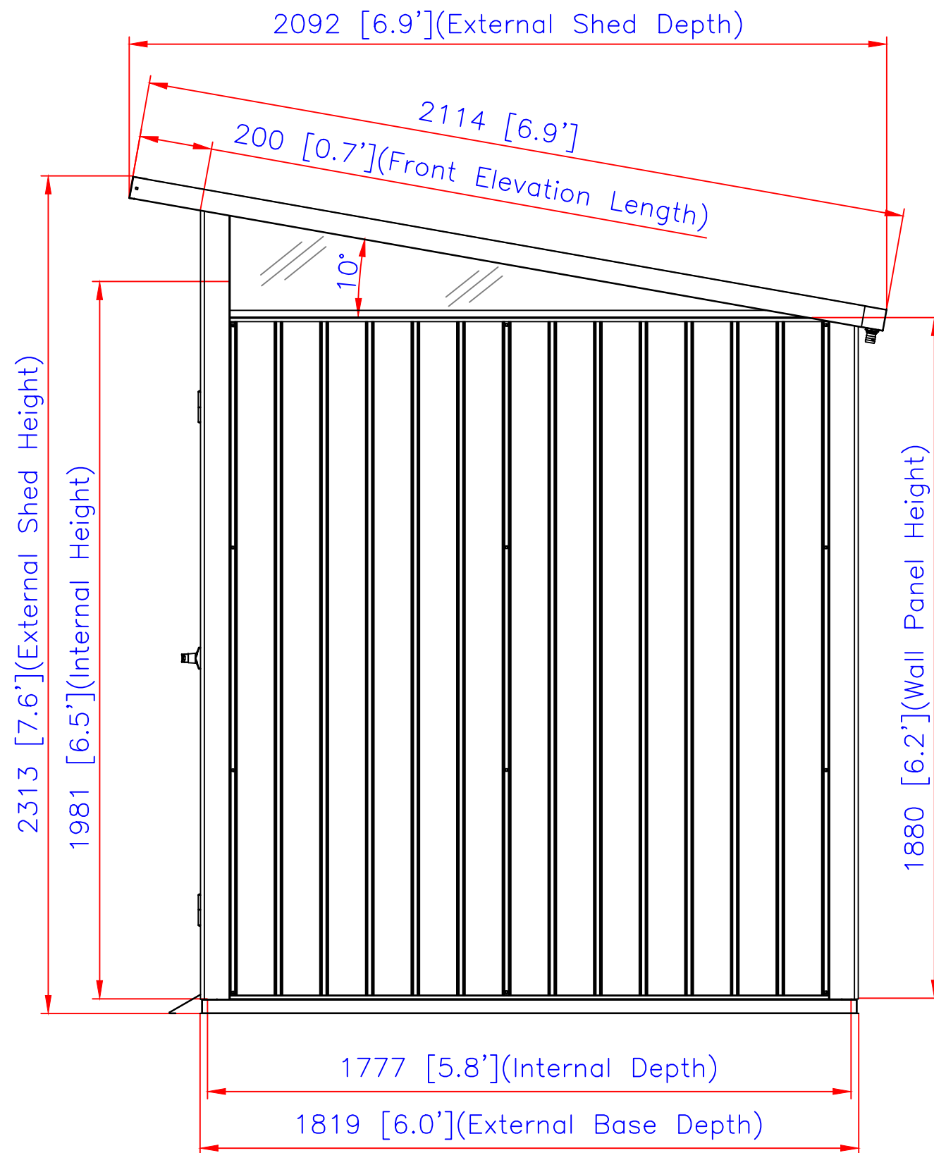
Side View
